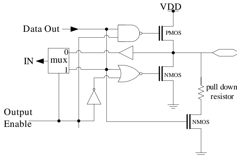
Figure 4-6 Block diagram of the PA port
