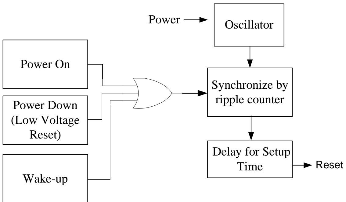
Figure 7-1 Scheme of the Reset Controller
